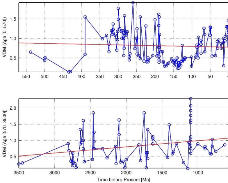
Figure 1. Dipole geomagnetic moment values during the time intervals from 0.570 Ga to present (above) and from 3.500 Ga to 0.570 Ga (below). The straight lines show the regression VDM = a \cdot t + b with numerical values for the slope a = (-0.00019 \pm 0.00028) \text{ Am}^2/\text{Ma} and a = (0.00019 \pm 0.00008) \text{ Am}^2/\text{Ma} for the Pz (Phanerozoic) and Arch+Ptz (Archean+Proterozoic) respectively (Schreider et al. 2019a,b)
